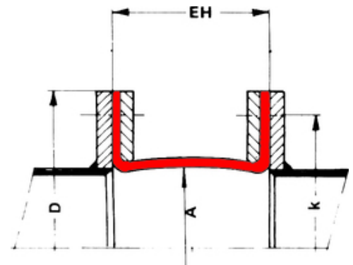
Note | Type 31 - Fabric Expansion Joint | dimensional sketch
