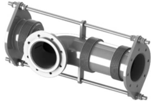
Note | Type MPB - Pressure Balanced Expansion Joint | 3D view
