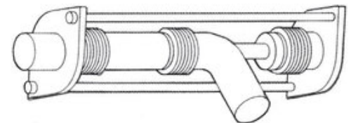
Note | Type MPB - Pressure Balanced Expansion Joint | sketch
